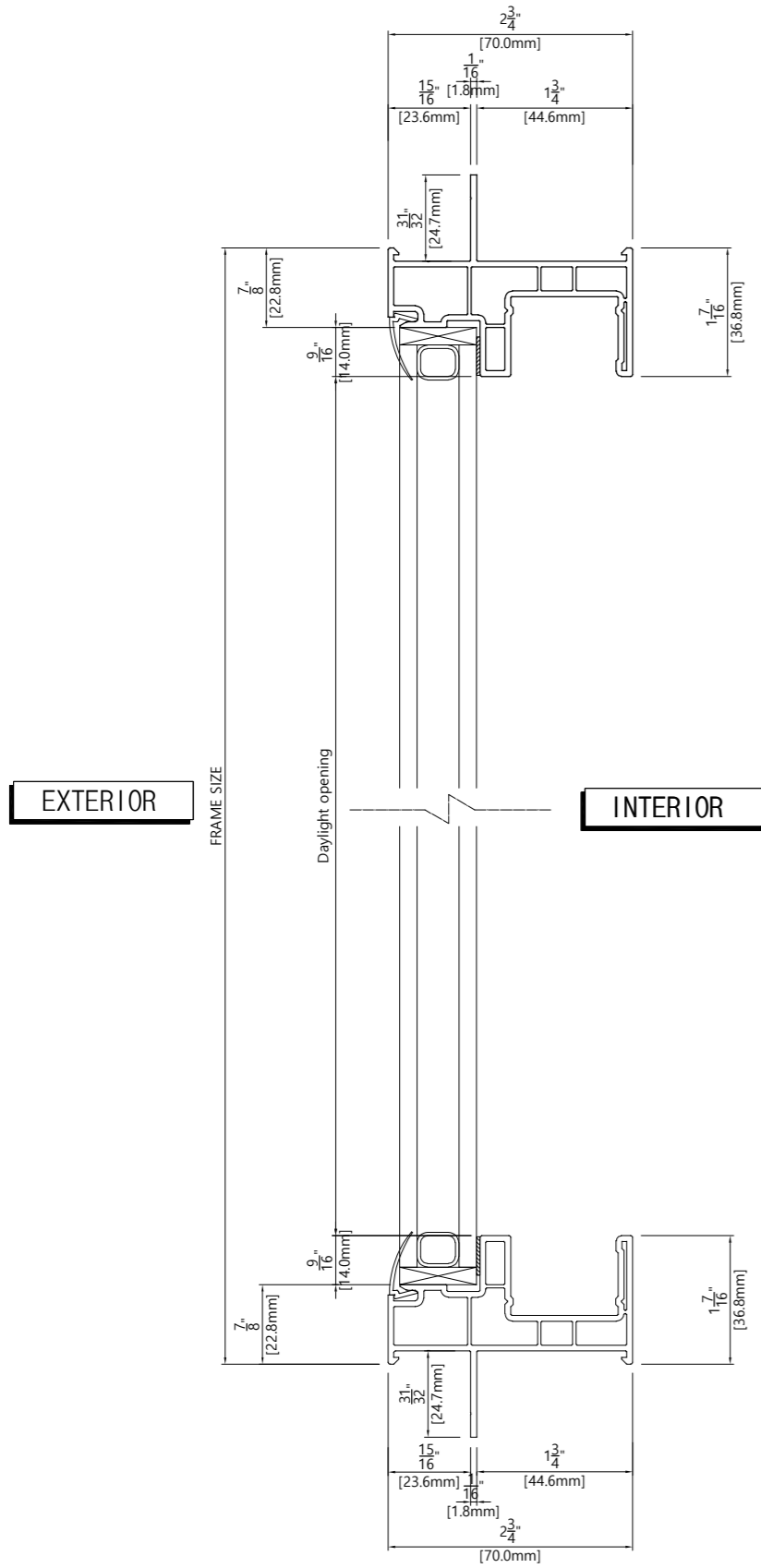
1 A-A' SECTION Head jamb and SILL
